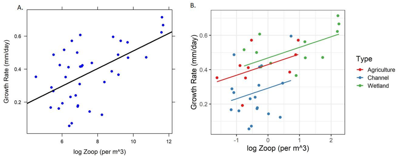
Figure 16. Relationships between caged fish mean daily growth rate (mm/day) and log zooplankton density (per m³). A. for all locations combined, and B. by habitat type. The dots represent the raw data, the black line shows a simple linear regression, and the colored lines show habitat specific daily growth rate predictions from the best mixed effects model.
