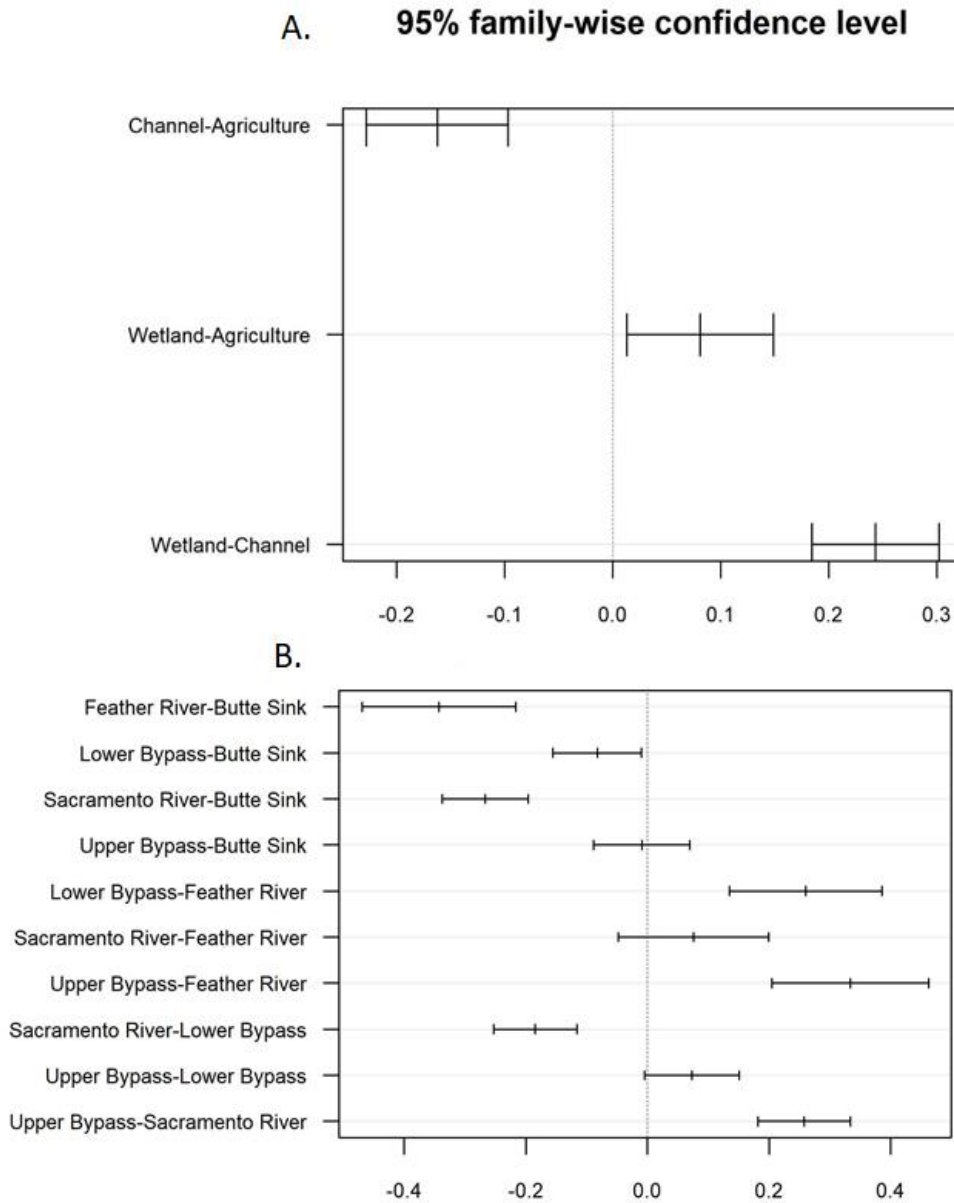
Figure 15. Pairwise comparison of mean daily growth rates (mm/day). A. for each habitat type. B. for each region. If a segment crosses the 0 vertical line, it means that the difference between growth rates is not statistically significant.
