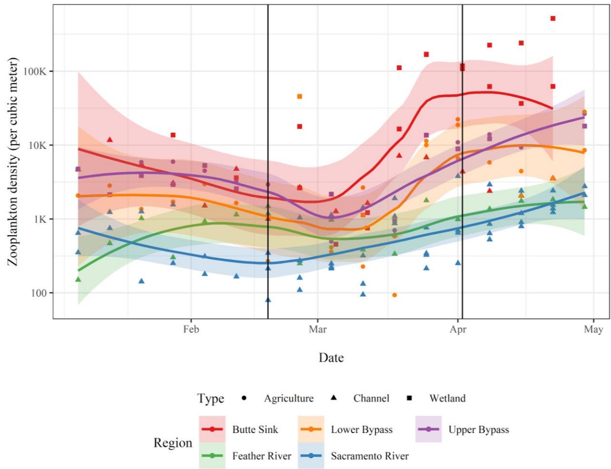
Figure 8. Total zooplankton density (per \text{m}^3 ), from ambient zooplankton sampling, summed for all taxa displayed on a log scale with trend lines for the different regions. The symbols represent zooplankton density for the different habitat types. The black vertical lines show the cage experiment time period.
